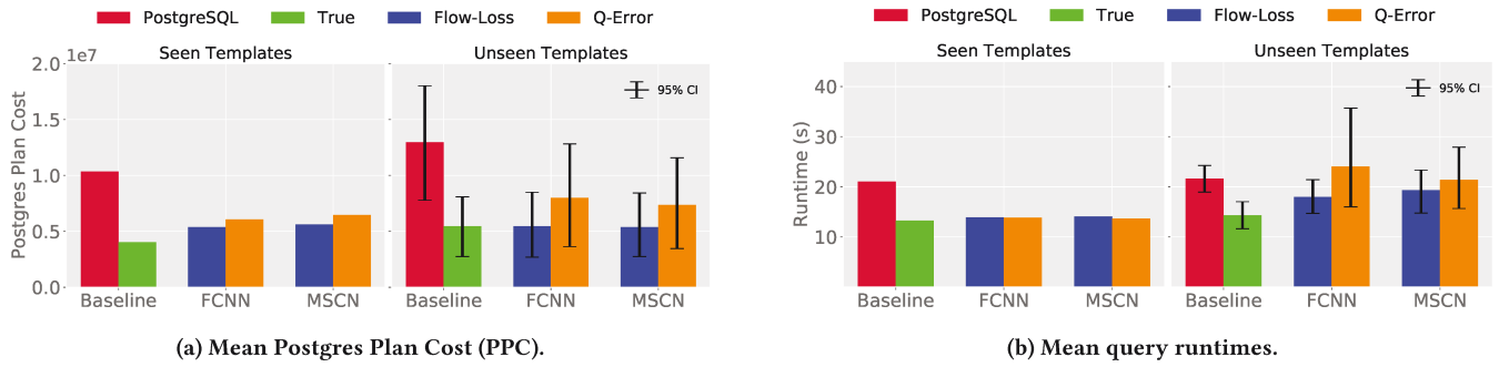
Figure 10: Comparing performance of all models on seen versus unseen templates. For unseen templates, we do ten experiments using ten different training/test template splits.
