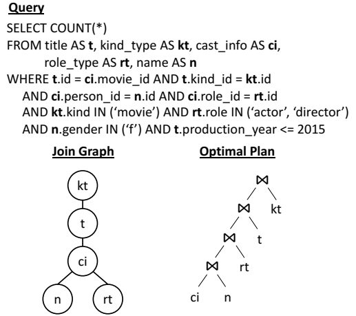
Figure 3: Join graph and optimal plan for sample query Q_1 on the IMDb database.
