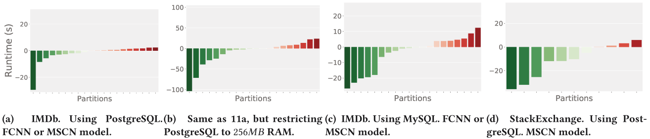
Figure 11: Each bar shows the mean runtime improvement (green) or regression (red) of Flow-Loss over Q-Error on a single unseen partition using the same model architecture. Lower is better for Flow-Loss models.
