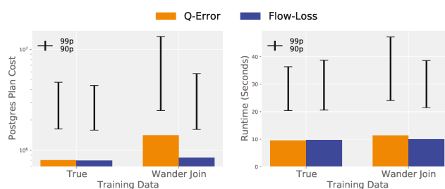
Figure 17: Mean PPC and runtimes, along with 90p to 99p error bars for a FCNN model trained with true or wander join cardinalities.
