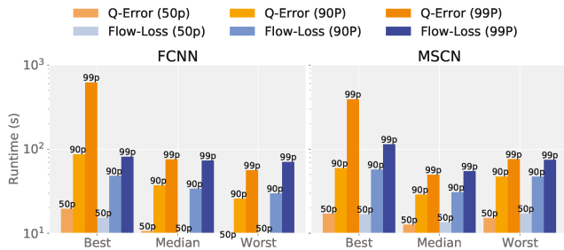
Figure 12: Best, median, and worst partition for Flow-Loss models by runtime difference from its corresponding Q-Error model on unseen template partitions for the FCNN architecture (left) and MSCN architecture (right) on the IMDb workload on PostgreSQL.
