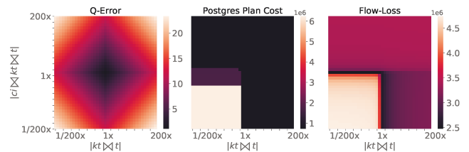
Figure 8: Comparing Q-Error, PPC, and Flow-Loss when we vary estimates of two sub-plans at the same time. The colors go from dark (low errors) to light (high errors).
