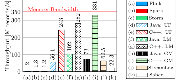
Figure 10: NYT query single node.
