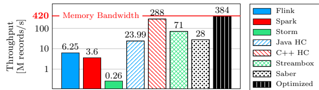
Figure 1: Yahoo! Streaming Benchmark (1 Node).
