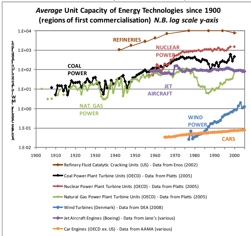
FIGURE 4. UP-SCALING IN SELECTED ENERGY TECHNOLOGIES SINCE 1900.
