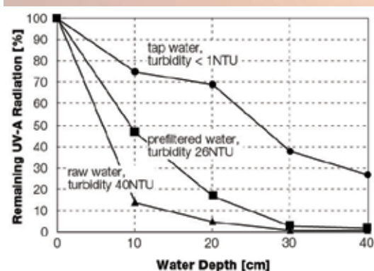
Figure 12: Reduction of UV-A radiation as a function of water depth and turbidity [16]
