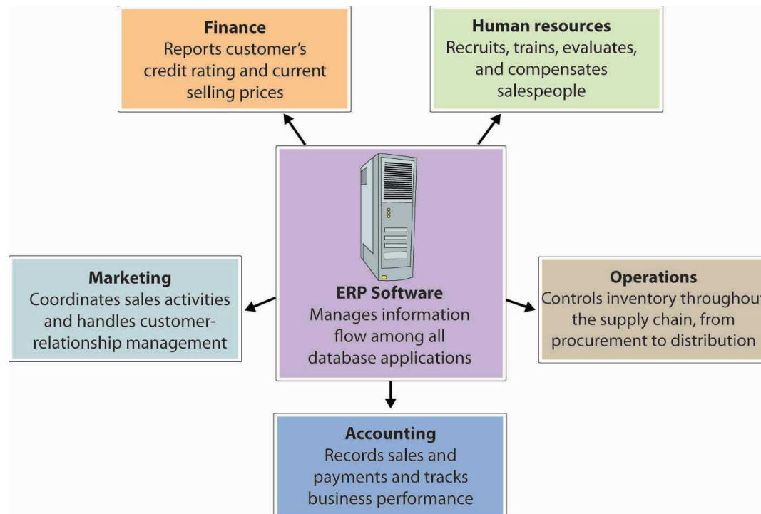
Figure 15.2 ERP System
