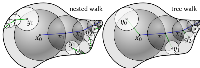
Fig. 10. Left : naïvely nesting a Poisson and Laplace estimator to solve a biharmonic equation yields a large number of walks. Right : by re-using the boundary path (blue) to compute source contributions (green), we obtain lower variance for the same total compute time.
