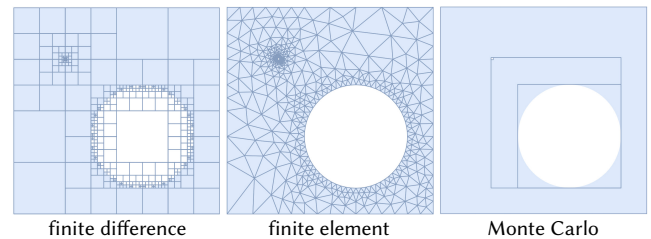
Fig. 23. Grid- and mesh-based algorithms (left, center) consume significant memory since they explicitly discretize even simple geometry, and must use gradual grading to maintain good element quality. Monte Carlo methods (right) concisely represent smooth geometry and small features via a bounding volume hierarchy (BVH), providing excellent memory scaling.
