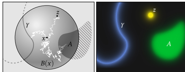
Fig. 9. Source terms can be importance sampled by randomly picking points on the source, restricted to the current ball in the walk. Without importance sampling, only the area source f_A would appear on the right; the point source f_z and curve source f_\gamma would never get sampled.
