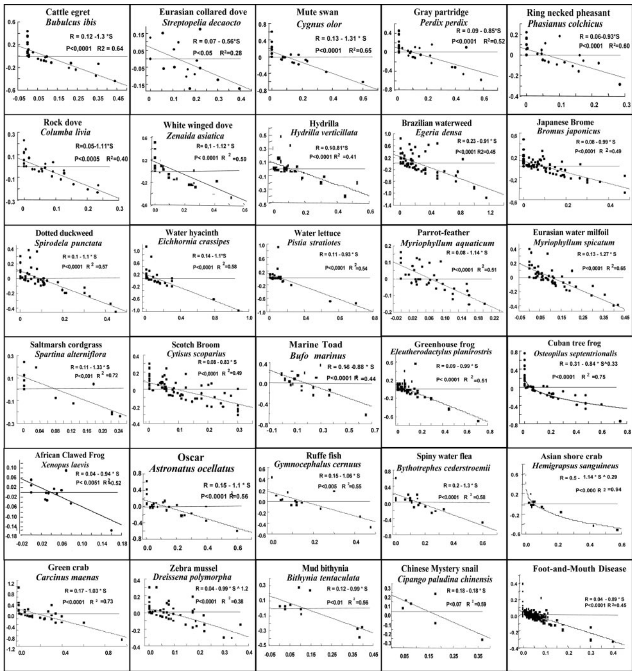
Fig. 2. Observed R -functions for the 30 taxonomically distinct organisms analyzed in this study. In all plots, the y axis is the rate of change in S (i.e., R_t ) and the x axis is S , as in Fig. 1. Estimated parameters, their statistical significance, and explained variance from the complete model are indicated within each plot. All cases indicate strong regulation of spread. Only two cases were best described by nonlinear R -functions (far right column, rows four and five).
