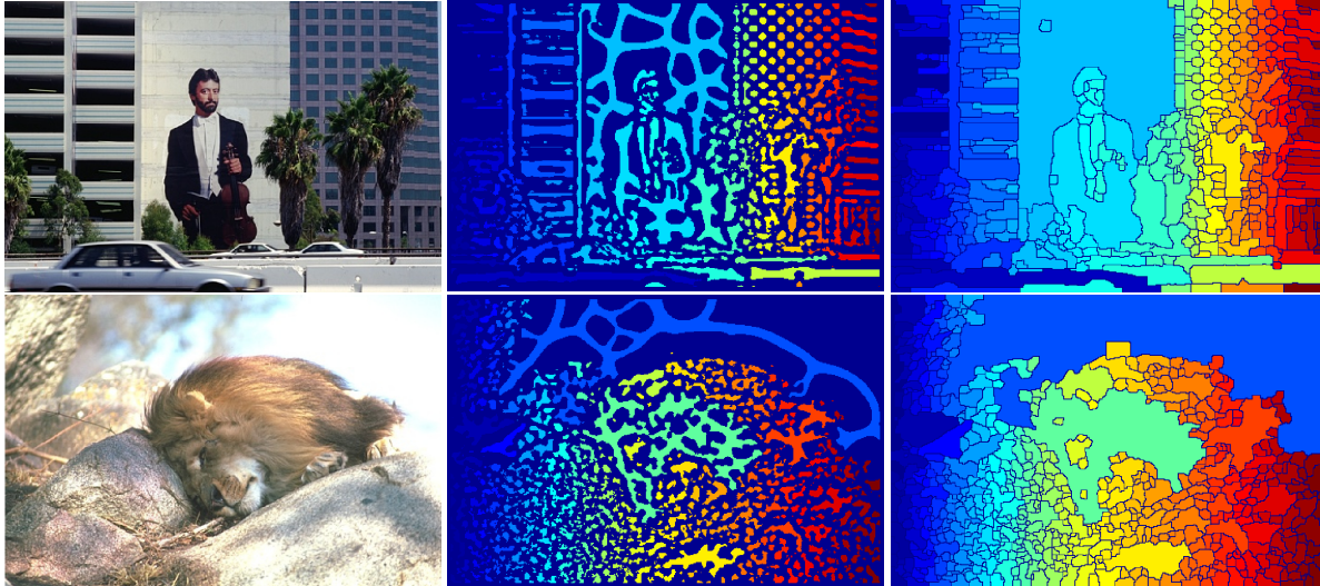
Figure 3: Seeds and segmentation. From left to right: original images, GVF based seeds obtained by thresholding the flux flow \mathcal{F} with \theta and the watershed segmentation. The color values denote different labels of the seeds and segments.
