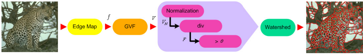
Figure 1: Overview of the processing pipeline for medial feature oversegmentation. The GVF field V is computed on the edge map. After normalization of V and the computation of the flux flow \mathcal{F} the seeds are obtained by thresholding with \theta . Starting from the seeds the watershed is computed using \mathcal{F} as a height map.
