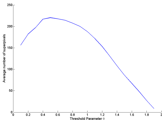
Figure 4: Influence of the thresholding parameter \theta on the number of generated superpixels (averaged over all images in the Berkeley Segmentation Dataset).
