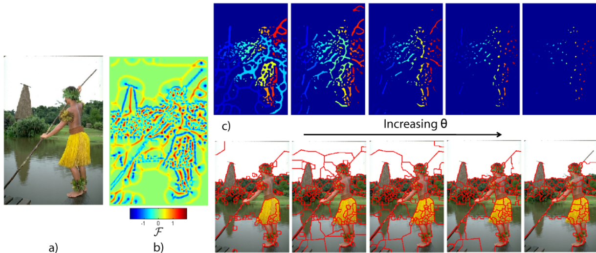
Figure 2: a) Original image b) Flux flow field \mathcal{F} c) Influence of the thresholding parameter \theta for the seeding on the resulting superpixel segmentations. From left to right parameter is set to (0.2, 0.5, 0.8, 1.1, 1.4). Top: \mathcal{F} > \theta , Bottom: Resulting oversegmentation.
