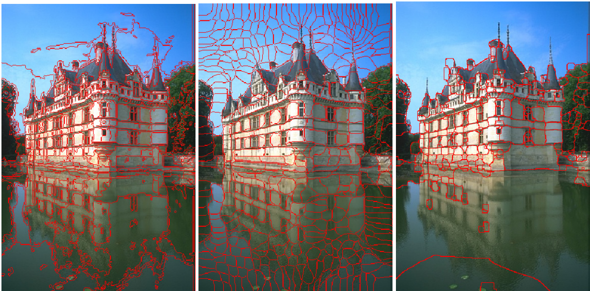
Figure 6: Experimental result on the example image from Figure 5. From left to right: segmentation obtained by superpixel algorithm after [4], segmentation obtained by superpixel algorithm after [10] and the oversegmentation result of our medial feature based approach.
