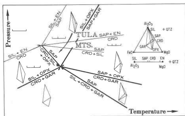
Fig. 10. Pressure-temperature diagram based on Schreinemaker's construction of phase relations in the systems \text{MgO-Al}_2\text{O}_3\text{-SiO}_2 (light lines) and \text{FeO-MgO-Al}_2\text{O}_3\text{-SiO}_2 (heavy lines). Compositional space for each system is shown on the right. Quartz is present in all assemblages. P - T conditions of metamorphism of rocks exposed in the Tula Mountains are indicated. Derivation of diagram is explained in text. Abbreviations: Crd = cordierite, Qtz = quartz, Sil = sillimanite, Sap = sapphirine, Opx = Orthopyroxene, En = enstatite, Gar = garnet. Curves for reactions \text{Crd} + \text{Sil} = \text{Sap} and \text{Crd} = \text{Sap} + \text{En} are shown divergent for illustration; in actuality, these curves are most likely almost coincident (Newton et al. , 1974).
