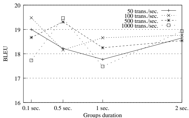
Figure 3: Comparison of different pruning configurations on the first pass.
