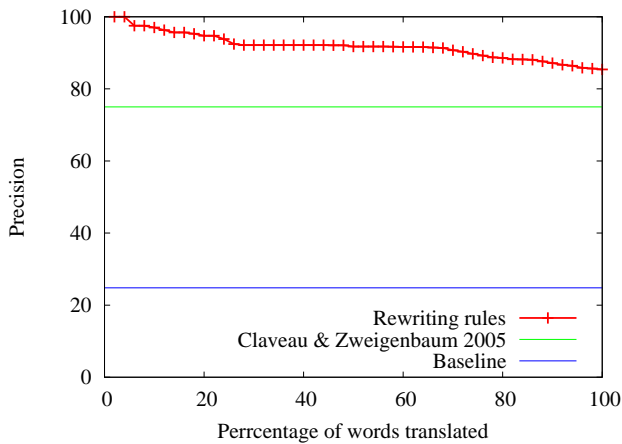
Figure 2: Performances of French into English translation
