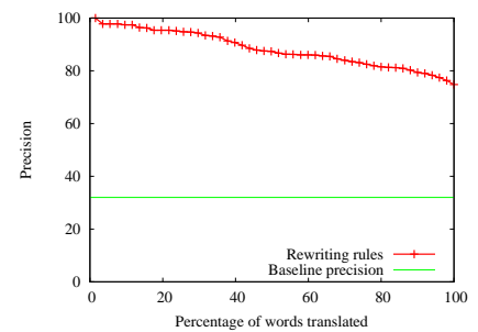
Figure 9: Performances of Czech into English translation
