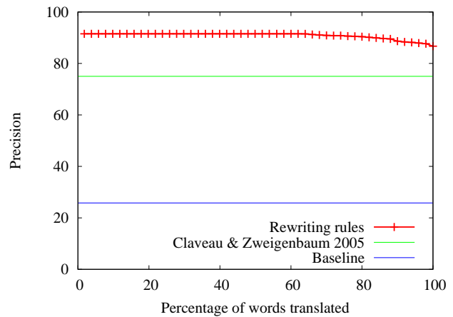
Figure 3: Performances of English into French translation
