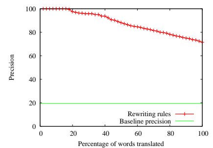
Figure 6: Performances of translation from Portuguese into English
