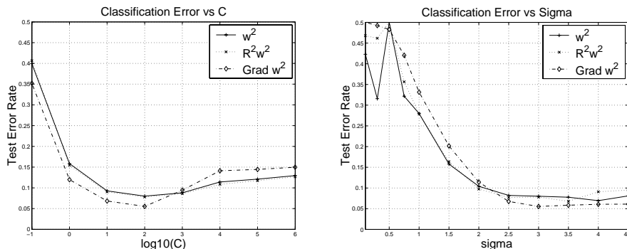
Figure 5: Plots of the influence of C and \sigma on the test error (averaged over 100 realizations) using the nonlinear toy dataset (training set size is 50). (left) Feature selection and classification error with \sigma = 3 vs C . (right) Feature selection and classification error with C = 100 vs \sigma .
