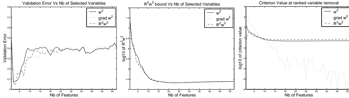
Figure 4: Different ways of choosing the number of ranked features to be provided to the predictor. Results for \|\mathbf{w}\|^2 , \nabla\|\mathbf{w}\|^2 and R^2\mathbf{w}^2 are depicted. (left) Validation error. (middle) L error Estimation with \frac{1}{m}R^2\mathbf{w}^2 . (right) Criterion value when variable has been removed.
