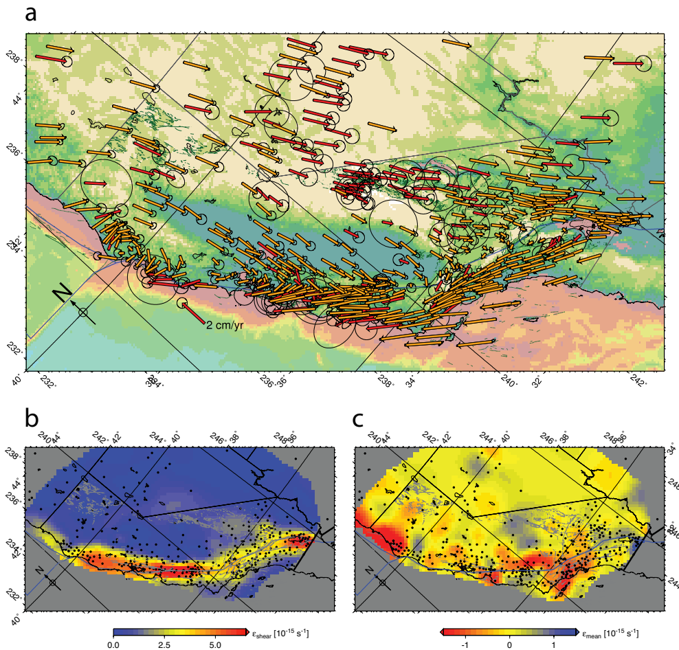
Plate boundary deformations, involving (a) surface velocities, (b) shear strains, and (c) mean strains, quantified here for the San Andreas system by geodetic measurements, provide a framework for stress accumulation and release, but the overall driving process and resulting earthquake stresses are not well understood. (Image modified from J.P. Platt, B.J.P. Kaus, and T.W. Becker, 2008. The mechanics of continental transforms: An alternative approach with applications to the San Andreas system and the tectonics of California, Earth and Planetary Science Letters , 274:380–391, doi:10.1016/j.epsl.2008.07.052.)
