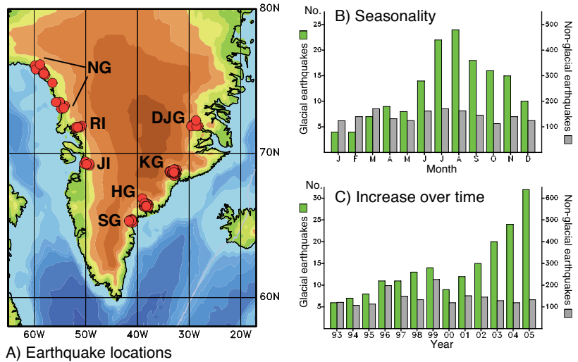
Example of novel glaciological signals studied with seismology. Seismically identified and located long-period glacial events detected with the GSN are associated with major outlet glaciers in Greenland, showing seasonality and annual variability. (Image from G. Ekström, M. Nettles and V.C. Tsai, 2006. Seasonality and increasing frequency of Greenland glacial earthquakes, Science , 311(5768):1756–1758, doi:10.1126/science.1122112. Reprinted with permission from AAAS.)
