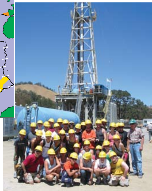
Students in the SCEC undergraduate internship programs visiting SAFOD site at Parkfield during its active drilling phase in 2004. (Figure courtesy of T. Jordan.)
