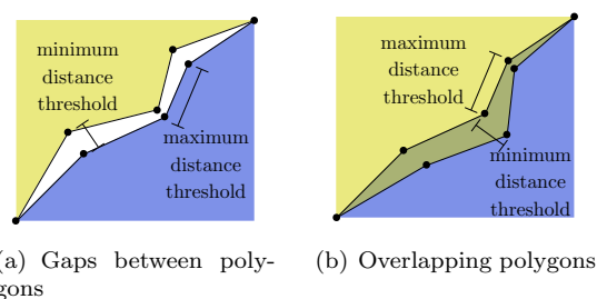
Figure 2: Defining a threshold for vertex, edge and face snapping. The threshold to use should be larger than the largest minimum distance between the matching boundaries, and smaller than the minimum distance between vertices.
