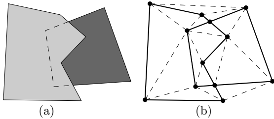
Figure 10: (a) Two overlapping polygons. (b) CGAL’s constrained triangulation of the polygons.
