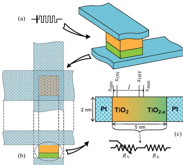
Fig. 2. Physical representation of memristor switching. (a) Memristor symbol and a 3-D view of the Pt/TiO 2 /Pt structure. (b) Top and side cross sections of the structure. (c) Switching behavior of the memristor, whereby “doped” and “undoped” regions correspond to R_{\text{on}} and R_{\text{off}} , respectively, being the two extreme states for the variable resistance R_V . Here, R_S is a series resistor around 200 \Omega [10]. The dopant consists of mobile charges. Assuming the tunneling [11], l introduces the initial (maximum) tunneling barrier width, bounded by two extremes ( x_{\max} ) and minimum ( x_{\min} ) possible positions, x indicates the position of the tunneling barrier. As an example, with x_{\max} = 19 \text{ \AA} and x_{\min} = 11 \text{ \AA} , we have l = 8 \text{ \AA} . At the same time, x_{\text{off}} and x_{\text{on}} are 18 \text{ \AA} and 12 \text{ \AA} , respectively.
