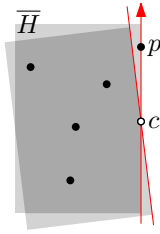
Figure 1: Illustration of the proof of Lemma 1.
