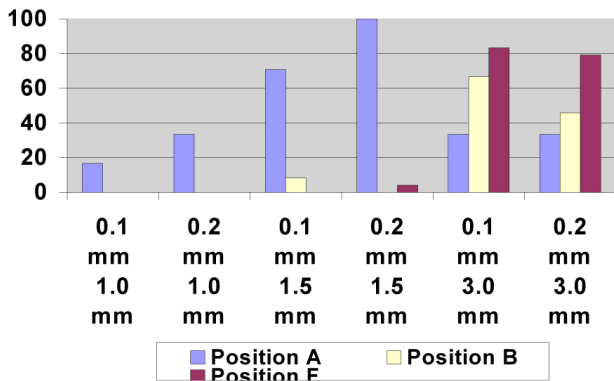
Figure 11: Results of the positions A, B and F (cf. Figure 7), tested with the big die. The x-axis lists the thickness of the metal foil (upper row) and the thickness of the spacer (lower row), e.g., the first bar on the left reflects the results with 0.1mm metal foil and 1.0mm spacer.
