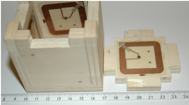
Figure 2: The large normal die with the lid open, revealing the enclosed RFID tags. The scale on the ruler is centimeter.
