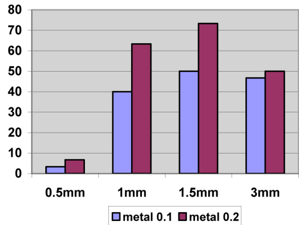
Figure 9: The results of the random rolls with the big die, depending on the thickness of the spacer (x-axis).
