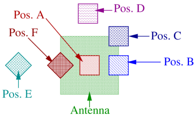
Figure 7: The different positions on the antenna that were tested to evaluate the homogeneity of the RF field.
