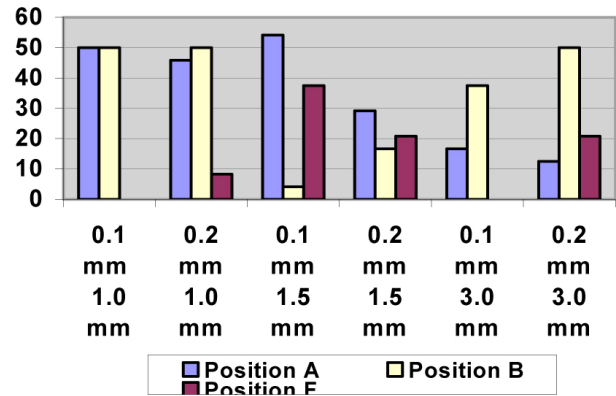
Figure 12: Results of the positions A, B and F (cf. Figure 7) using the small die. The x-axis lists the thickness of the metal foil (upper row) and the thickness of the spacer (lower row), e.g., the first bar on the left reflects the results with 0.1mm metal foil and 1.0mm spacer.
