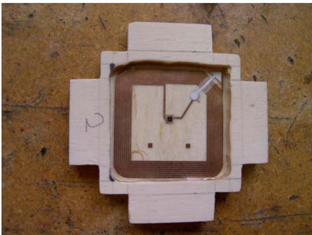
Figure 3: One side of the milled-out die disclosing the attached RFID tags.
