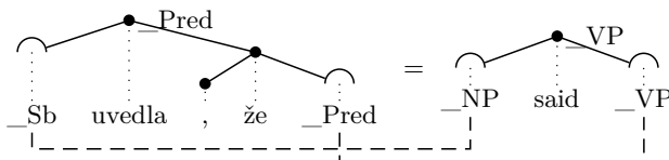
Figure 4. A sample analytical treelet pair.
