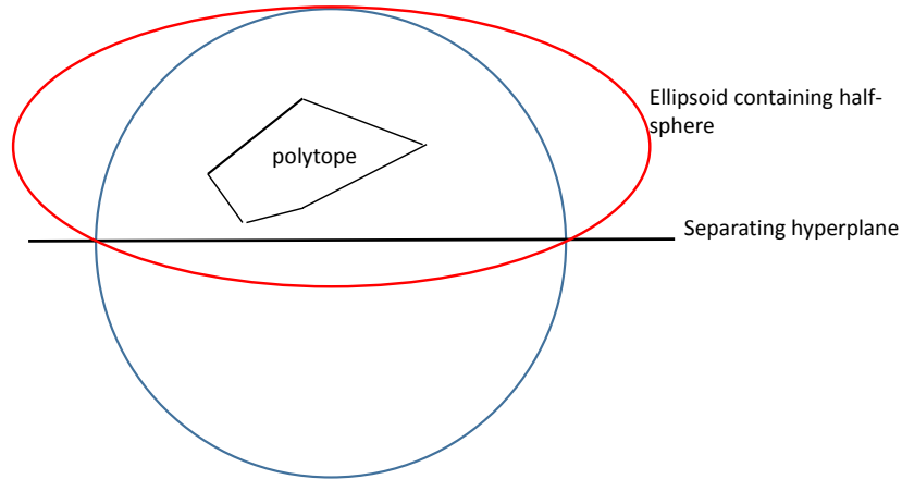
Figure 10.7: Ellipsoid Algorithm
