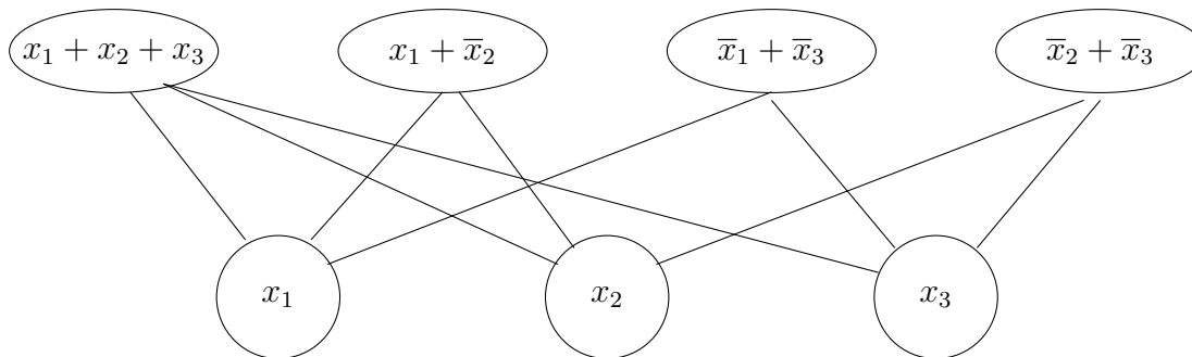
Figure 9.3: The factor graph for the function
