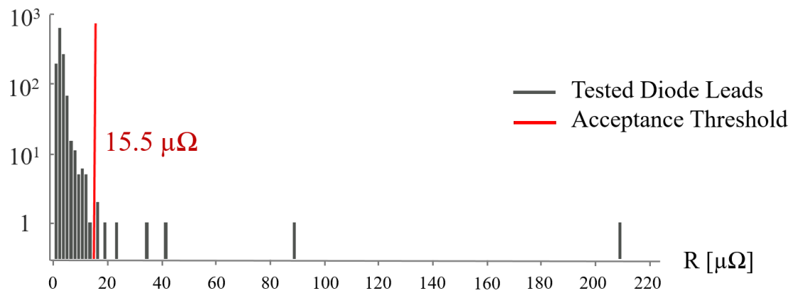
Figure 3.6: Diode bypass resistance data from 4 of the 8 main dipole circuit. Note that several bypasses exceed the resistance thresholds with one even being measured at 14 times the limit. Data courtesy of M. Bednarek [75].
