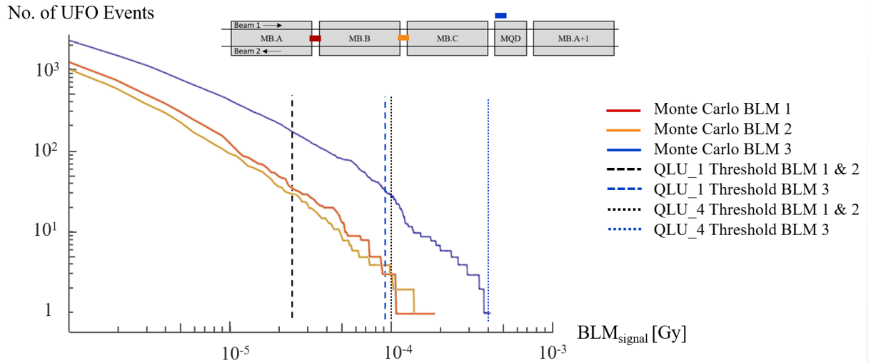
Figure 5.14: 6.5 TeV Monte-Carlo simulation results including quench limits for conservative and progressive QLU factors. Insert shows the corresponding BLM locations – Run 2.
