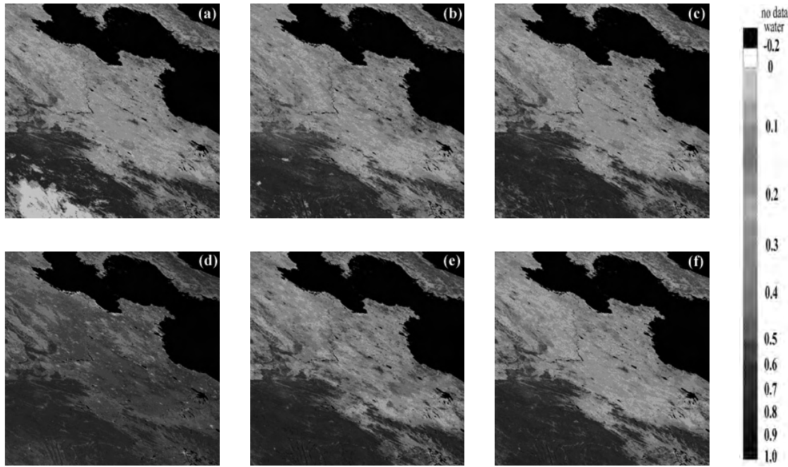
Figure 7. Compositd NDVI images at (a) data day 297, (b) data day 305 and reconstructed time series at data day 297 generated by (c) the BISE method, (d) the weighted Fourier series fitting method, (e) the S-G filter method, and (f) the wavelet method. A color version of this figure is available at the ASPRS website: www.asprs.org .
