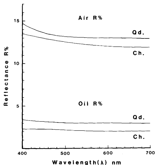
FIG. 3. Reflectance curves in air and oil of qandilite compared with chromite (IMA/COM. data file no: 1600). Qd = qandilite and Ch = chromite.
