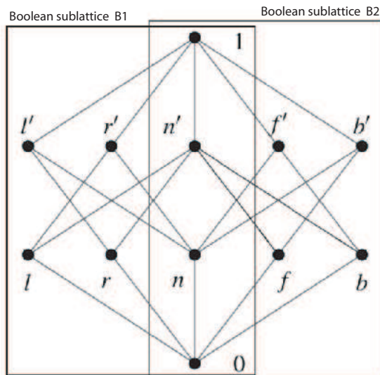
Figure 1: Hasse diagram for L_{12} . The boolean sublattices B1 and B2 corresponding to the two complementary contexts are indicated by squared lines.
