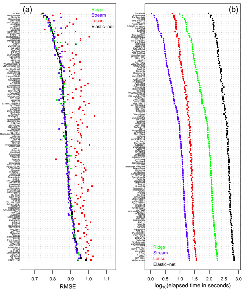
Fig. 2. Predictive performance and computation time for the Sanger cell line panel. Results for each compound.
