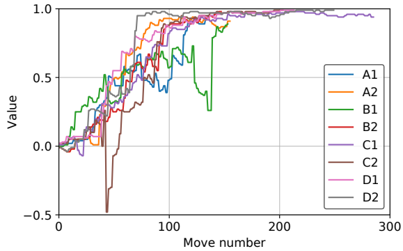
Figure 1. Predicted values after each move for 8 selected games versus human professional players (2 games per player). A positive value indicates that the model believes it is more likely to win than the human. Per players’ request, we anonymize the games by arbitrarily labeling the players with letters ‘A’ to ‘D’.
