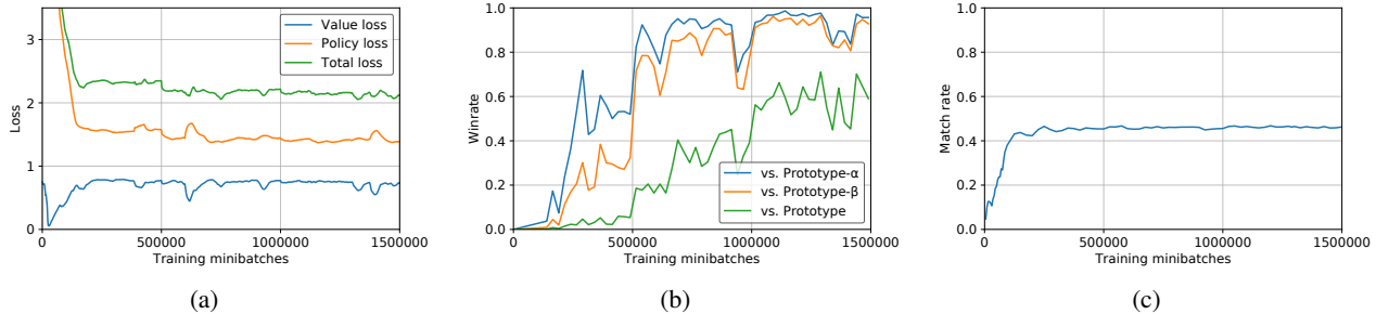
Figure 3. (a) Model’s training loss (value, policy, and sum) during training. (b) Win rates vs. the prototype model during training. (c) Match rate between trained model and human players on moves from professional games (as described in Appendix B.1). The learning rate was decreased every 500,000 minibatches.
