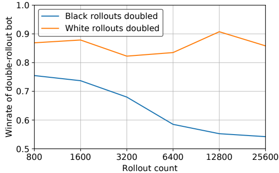
Figure 7. Win rate when playing with 2x rollouts against the same model with 1x rollouts.
