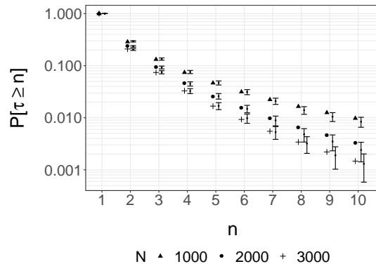
Figure 4: Empirical estimates of \mathbb{P}[\tau \geq n] (with \pm 2 standard errors) and comparison with those implied by the large sample approximation for stochastic kinetic model.
