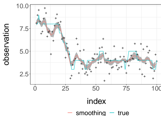
Figure 5: Unbiased estimates of \mathbb{E}(X_{1,t} | y_{1:T}) (red) (with \pm 3 pointwise standard errors) and X_{1,t} (blue) for Markov jump process.
