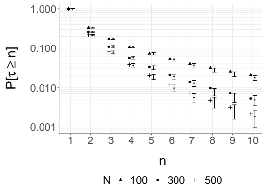
(a) Empirical ( \pm 2 standard errors) and predicted tail probabilities implied by large-sample approximation \mathbb{P}[\tau \geq n] .
