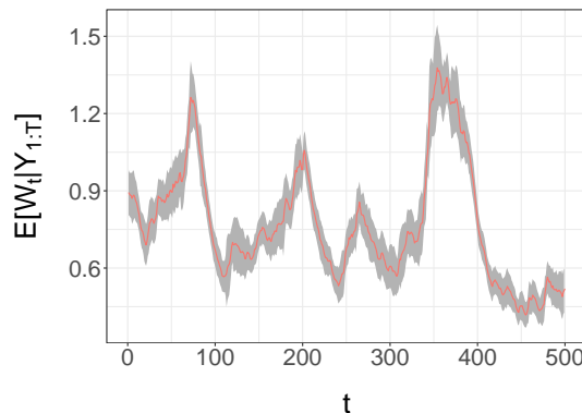
(c) Unbiased estimates of \mathbb{E}(W_t | y_{1:T}) of the S&P 500 over 2005–2007 and confidence intervals at \pm 3 standard errors.
