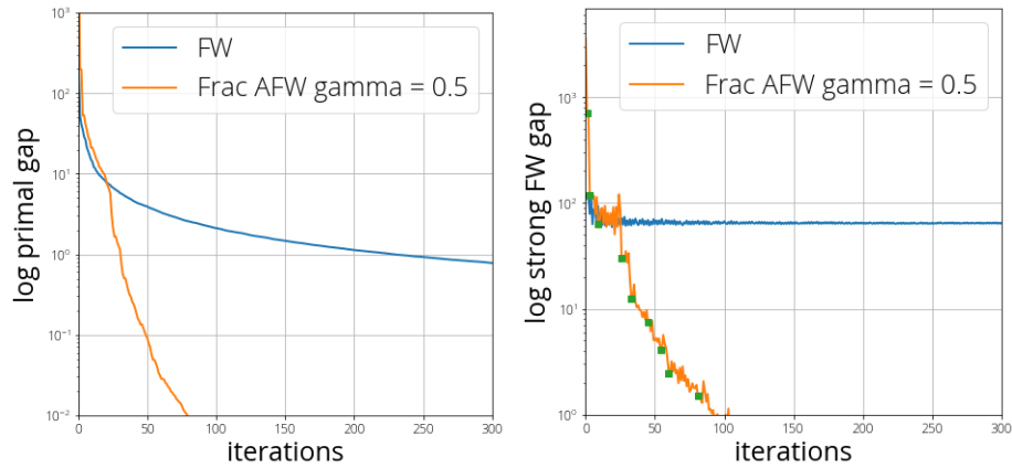
Figure 2: Comparing classical FW and Algorithm 1 with \gamma = 0.5 on regression problem (23) with \alpha = 1.5 , so that the classical geometric strong convexity condition does not hold. Green squares indicate restart times.
