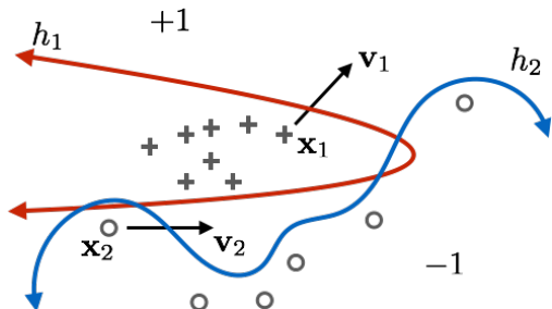
Figure 2: Two nonlinear decision boundaries, h_1 (red) and h_2 (blue). The instances with label +1 are marked by pluses, those with label -1 are marked by circles. An adversarial direction for h_1 at \mathbf{x}_1 is denoted by \mathbf{v}_1 , while an adversarial direction for h_2 at \mathbf{x}_2 is denoted by \mathbf{v}_2 .
