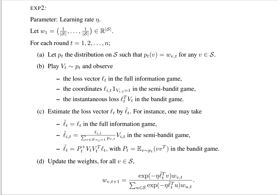
Figure 4: EXP2 forecaster.
