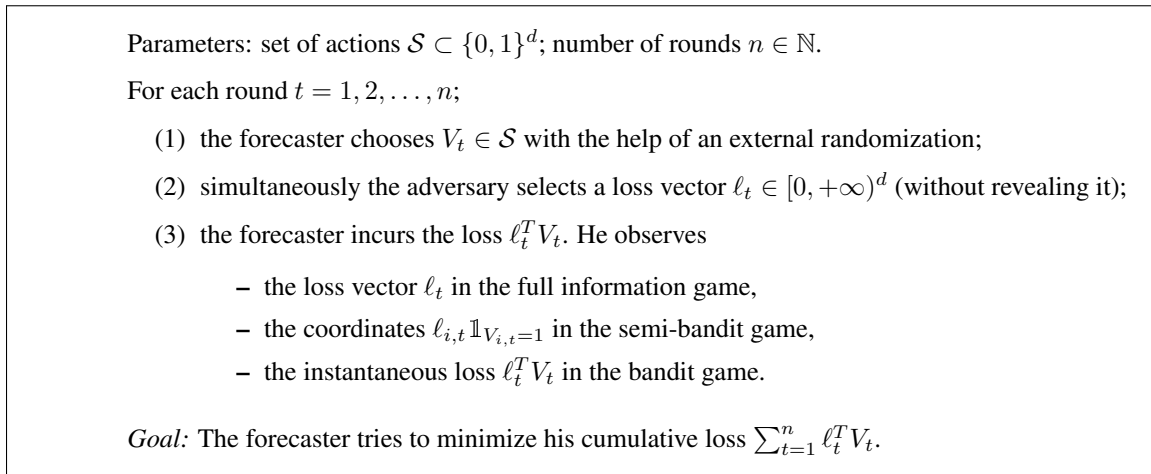
Figure 1: Combinatorial prediction games.
