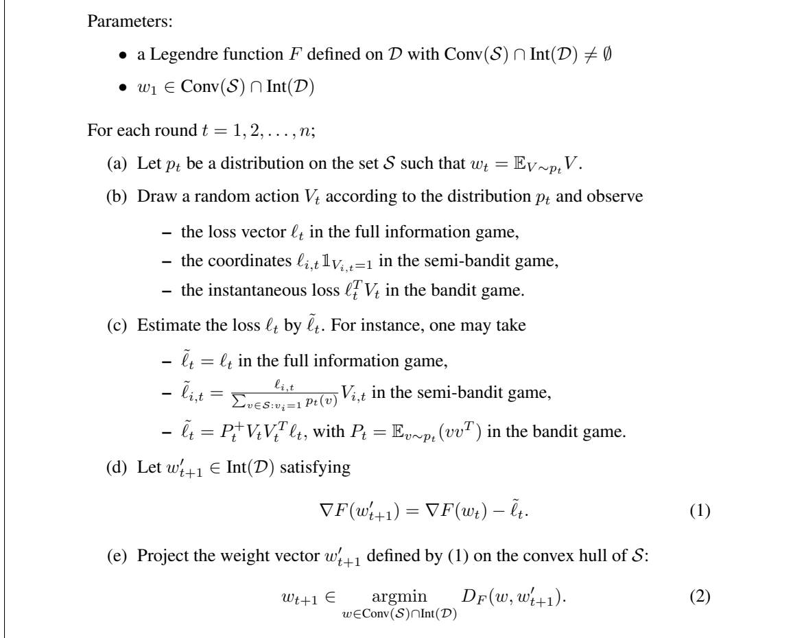
Figure 2: Combinatorial learning with Bregman projections (CLEB).
