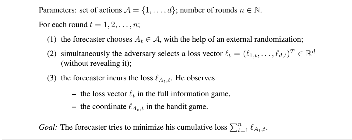
Figure 5: Standard prediction games.
