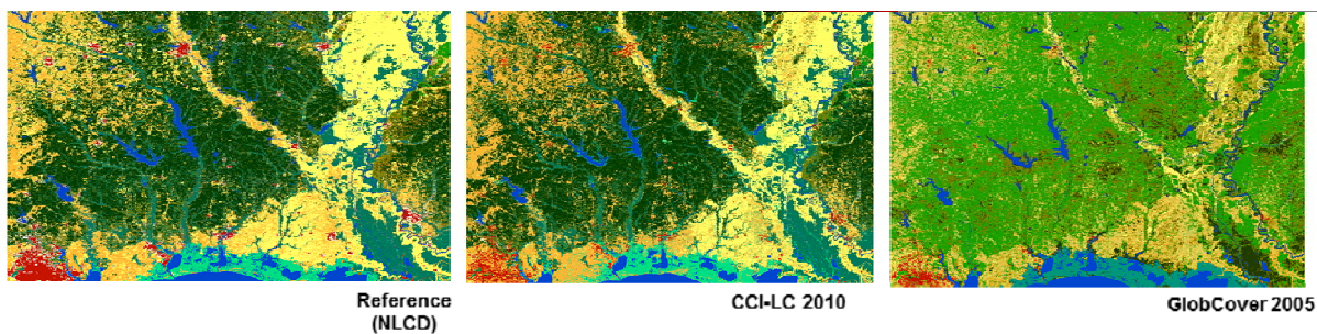
Figure 4-4: Comparison, in Florida (US), of the CCI-LC for the 2010 epoch (center) with the reference dataset used in the classification made of the US-NLCD (left) and the GlobCover 2005 product (right).
