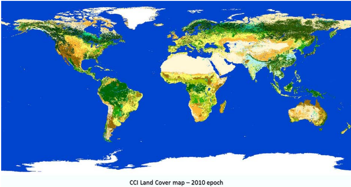
Figure 4-1: The CCI global LC map from the 2010 epoch (2008-2012), at 300m spatial resolution.
