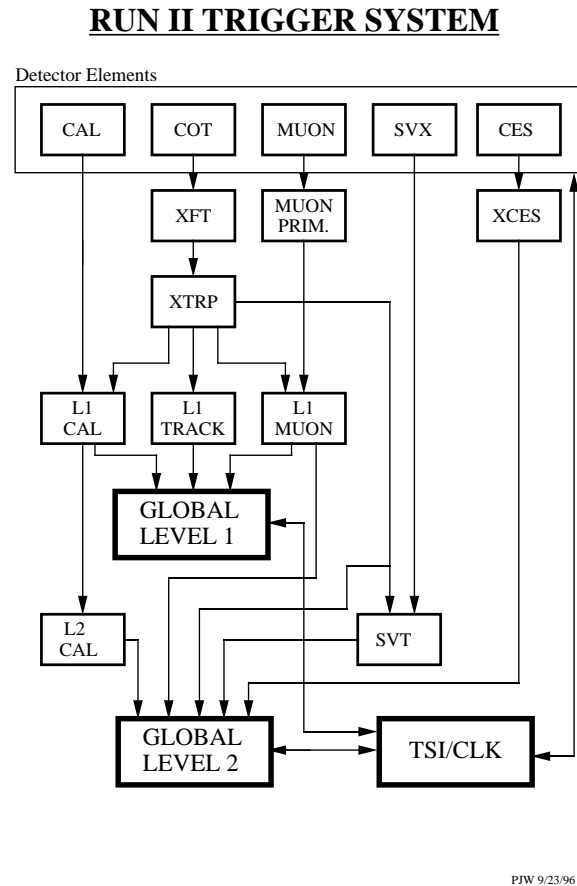
Figure 3.23: Block diagram of the Run II trigger system.
