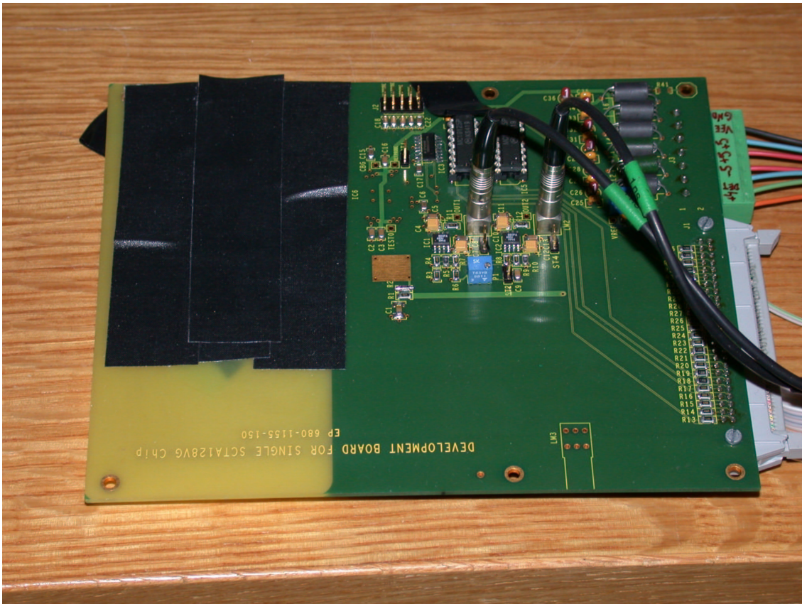
Figure 6.8: Single chip tests (the chip is in a protected space underneath the PCB).
