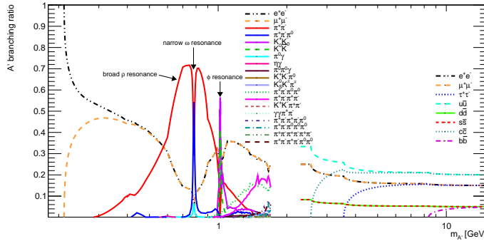
[t] Figure 7.11: Branching ratios of a kinetically mixed dark photon A' as a function of m_{A'} [587].
