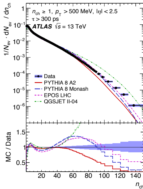
Figure 7.8: Charged particle multiplicities measured in minimum bias events with the ATLAS detector for events with at least one track with a minimum p_T of 500 MeV and |\eta| < 2.5 [582].
