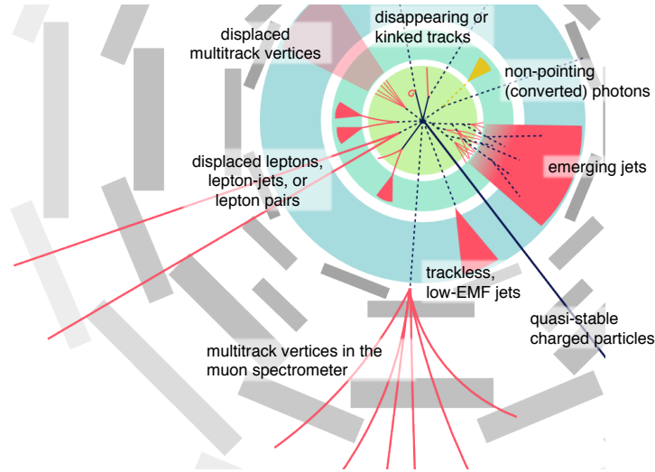
Figure 1.2: Schematic of the variety of challenging, atypical experimental signatures that can result from BSM LLPs in the detectors at the LHC. Shown is a cross-sectional plane in azimuthal angle, \phi , of a general purpose detector such as ATLAS or CMS. From Ref. [3].
