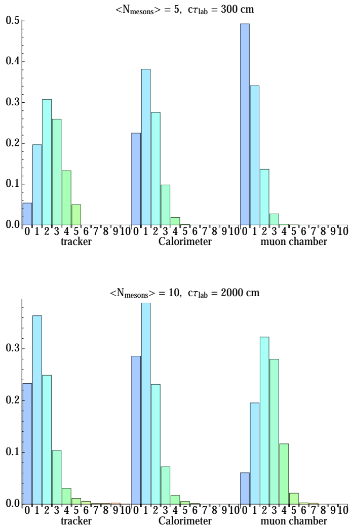
Figure 7.7: Distribution of decays occurring in the various detector elements, for those events with more than three decays occurring in the fiducial volume.
