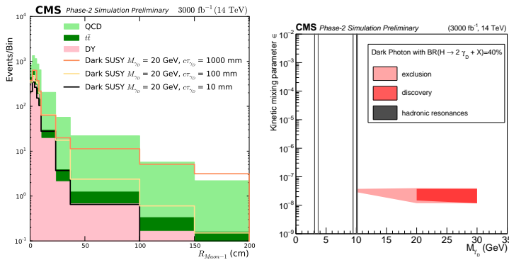
Figure 5.17: Left: Distance of the closest approach of the displaced muon track with maximum p_T to the primary interaction vertex, R_{\text{Muon}-1} , for signal and background after the final event selection. Right: Parameter scan in the \epsilon - m_{\gamma_D} plane. The grey lines indicate the regions of narrow hadronic resonances where the analysis does not claim any sensitivity [356].
