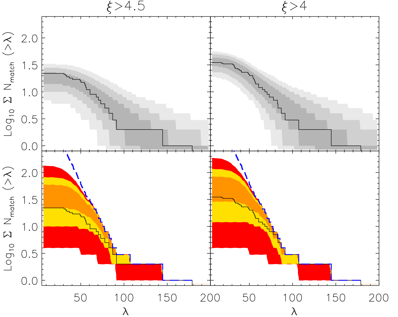
Figure 5. Consistency tests of our model (Section 3) and the SPT-SZ+RM catalog from the \sim 124 \text{ deg}^2 SPT-E field. The solid black lines show the observed cumulative distribution in richness \lambda of the \xi > 4.5 (left) and \xi > 4 (right) SZE-selected samples. Upper panels: Gray scale regions show 1, 2, and 3\sigma regions predicted by drawing 10^6 SZE-selected samples from the mass function and assigning \lambda according to our scaling relation constraints. There is good agreement with the data. Lower panels: Dashed blue lines show the cumulative distribution in \lambda of the full RM sample. Orange, yellow, and red areas define 1, 2, and 3\sigma regions representing the predicted cumulative distribution of the SPT-SZ+RM catalog using as input the full RM sample and the probability (Eq. 10) that each RM cluster will have an SPT-SZ counterpart, given our scaling relation constraints.
