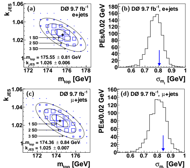
FIG. 25: (a) Two-dimensional likelihood \mathcal{L}(\mathbb{X}_N; m_t, k_{\text{JES}})/\mathcal{L}_{\text{max}} for data in the e +jets final state. Fitted contours of equal probability are overlaid as solid lines. The maximum is marked with a cross. (b) Distribution in expected uncertainty on m_t in e +jets final states, obtained using PEs where the t\bar{t} contribution is taken at m_t^{\text{gen}} = 172.5 GeV and k_{\text{JES}} = 1 , after calibration. The observed statistical uncertainty in data is indicated by the arrow. (c) Same as (a), but for the \mu +jets channel. (d) Same as (b), but for the \mu +jets channel.
