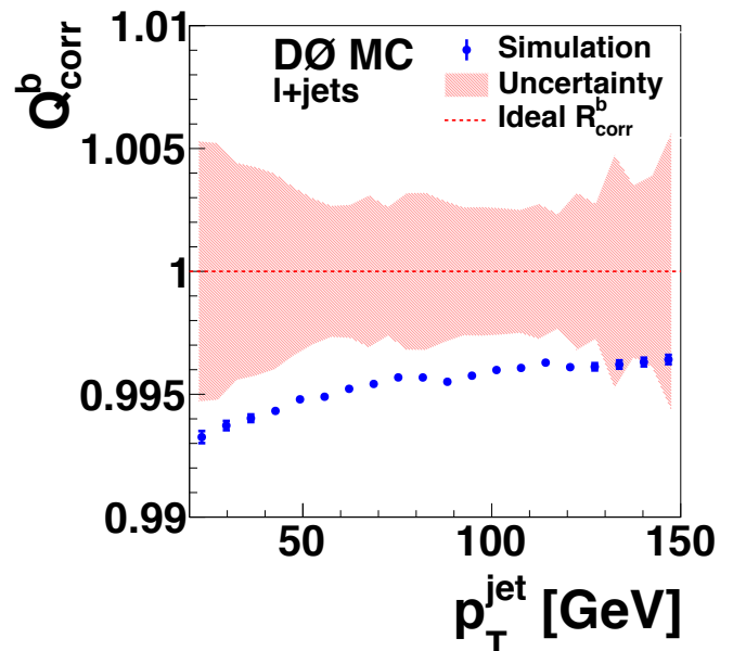
FIG. 32: The ratio Q_{\text{corr}}^b = F_{\text{corr,ALPGEN+HERWIG}}^b / F_{\text{corr,ALPGEN+PYTHIA}}^b for b -quark jets in simulated t\bar{t} events and \ell +jets final state as a function of the p_T of the jet. The ideal Q_{\text{corr}}^b of unity is indicated as the broken line. The uncertainties on the points reflect the finite size of the MC sample. The total uncertainty on the standard flavor-dependent correction for ALPGEN+PYTHIA is indicated as the band around unity.
