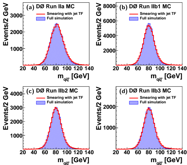
FIG. 7: Invariant mass of the dijet system matched to the W \rightarrow q\bar{q}' decay for (a) Run IIa, (b) Run IIb1, (c) Run IIb2, and (d) Run IIb3. Fully simulated jet-parton matched MC events passing all selection requirements are compared to partons with energies smeared using the jet TF, and then applying the same standard event selection criteria.
