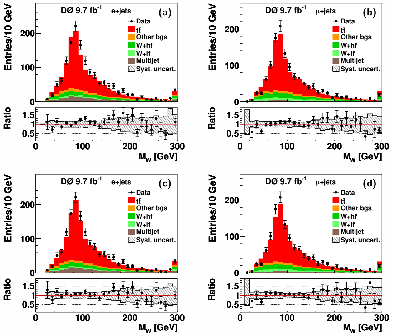
FIG. 27: Same as Fig. 26, but for the invariant mass of the dijet system matched to the W boson, assuming m_{\tilde{t}}^{\text{gen}} = 172.5 GeV, k_{\text{JES}} = 1 , and \sigma_{\tilde{t}\tilde{t}} = 7.24 pb ^{-1} [40] in the (a) e +jets and (b) \mu +jets final states, and for m_{\tilde{t}}^{\text{gen}} = 175 GeV, k_{\text{JES}} = 1.025 , and f corresponding to their measured values in the (c) e +jets and (d) \mu +jets final states.
