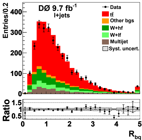
FIG. 33: The ratio R_{bq} = (p_T^{b_1} + p_T^{b_2}) / (p_T^{j_1} + p_T^{j_2}) for events with \geq 2 b -tagged jets, and R_{bq} = 2p_T^b / (p_T^{j_1} + p_T^{j_2}) for events with one b -tagged jet, after all selections. The category “Other bgs” encompasses Z +jets, WW , WZ , ZZ , and single top quark production, as well as dileptonic t\bar{t} decays. The production of a W boson in association with at least one b or c quark is denoted as “ W + hf ”, while “ W + lF ” stands for all other flavor configurations. The last bin includes overflow events. The ratio shows the number of observed events divided by the number of expected events in a given bin. The band of systematic uncertainty is indicated as a shaded area in the ratio plots, and includes dominant sources: JES, jet energy resolution, jet identification, flavor dependence of the detector response, and b tagging.
