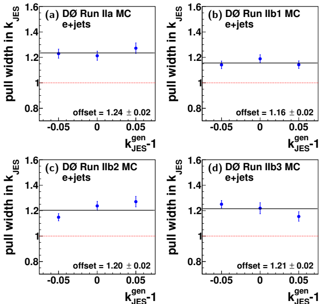
FIG. 17: The width of the distribution of the pull in k_{\text{JES}} , derived using simulations at each k_{\text{JES}}^{\text{gen}} point, as a function of k_{\text{JES}}^{\text{gen}} for (a) Run IIa, (b) Run IIb1, (c) Run IIb2, and (d) Run IIb3 in the e +jets final state. The error bars are given by the uncertainty on the width of the distribution in \pi_{k_{\text{JES}}} , which is not corrected for the effect that the same event can appear in many PEs, and therefore somewhat underestimated. The pull is fitted with a constant shown as a solid black line, whose value is given at the bottom of the plots. The broken line represents the case of ideal pull width of unity.
