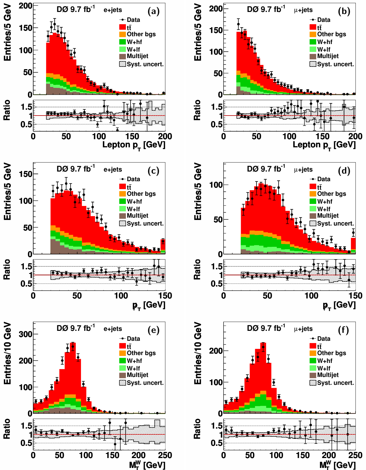
FIG. 29: Same as Fig. 28, but for the transverse momentum of the (a) electron or (b) muon, for the missing transverse momentum in (c) e+jets and (d) \mu+jets final states, as well as for the transverse mass of the W \rightarrow \ell\nu_\ell decay in (e) e+jets and (f) \mu+jets final states.
