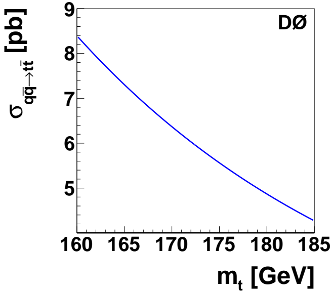
FIG. 1: The total partonic cross section for t\bar{t} production in p\bar{p} collisions through quark-antiquark annihilation at LO, as defined in Eq. (10).
