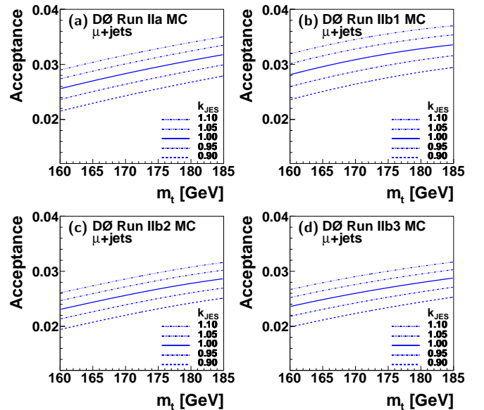
FIG. 3: Same as Fig. 2, but for the \mu +jets final state for (a) Run IIa, (b) Run IIb1, (c) Run IIb2, and (d) Run IIb3.
