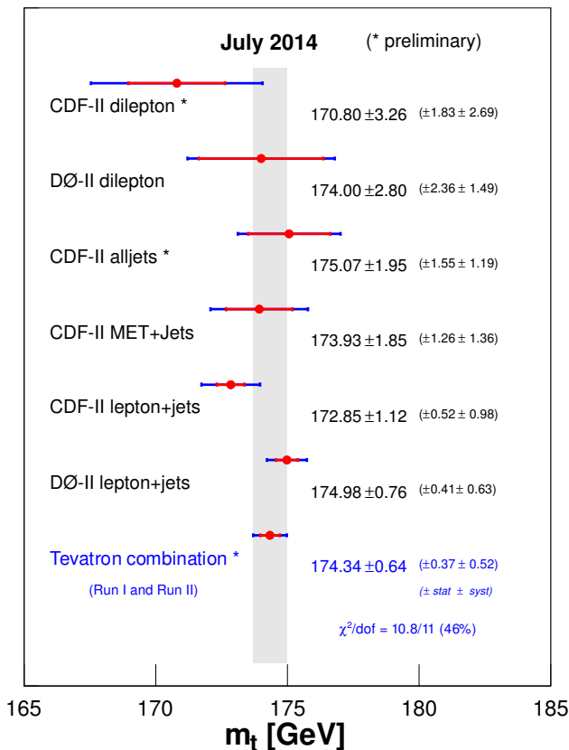
FIG. 34: Summary of the measurements performed in Run II of the Tevatron which are used as inputs to the Tevatron combination [8]. The inner error bars indicate the statistical uncertainties, while the outer bars represent the total uncertainties. The Tevatron average value of m_t obtained using input measurements from Run I and Run II is given at the bottom and its uncertainty is shown by the band. The Figure is adapted from Ref. [8].
