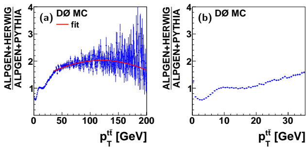
FIG. 31: (a) The ratio of predicted differential cross sections from ALPGEN+HERWIG to those from ALPGEN+PYTHIA as a function of p_T^{tt} at particle level. Also shown is the fit with a second-order polynomial used for reweighting ALPGEN+PYTHIA events in p_T^{tt} for 35 \text{ GeV} < p_T^{tt} < 200 \text{ GeV} . Below that range the reweighting is performed according to the histogram, and above with a constant factor of 1.67. Uncertainties are only statistical. (b) Same ratio in the range p_T^{tt} < 35 \text{ GeV} .
