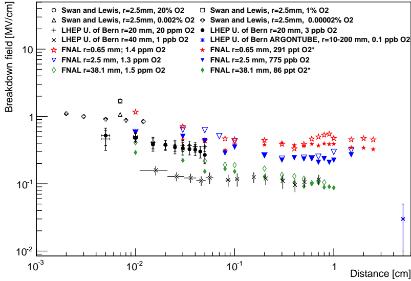
Figure 5. A comparison of the several measurements of the magnitude of the electric field at breakdown in liquid argon [20, 8]. The data points from Fermilab result from the highest and lowest contamination level measurement taken with each probe. The oxygen values with an asterisk are extrapolated from purity monitor measurements.
