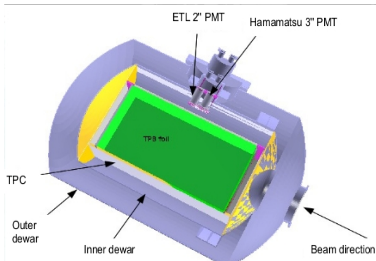
Figure 25. 3D CAD model cutaway of LArIAT system with wavelength-shifter-lined TPC walls and PMTs (and SiPMs, not shown) viewing the interior volume.
