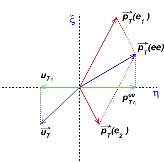
FIG. 7: (color online). Definitions of the \eta and \xi axes in Z \rightarrow ee events, and the dielectron and the hadronic recoil system projections in these axes. The \eta - \xi plane is transverse to the beam.
