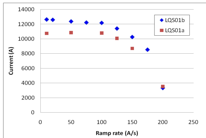
Fig. 5. LQS01a and LQS01b ramp rate dependence at 4.5K.
