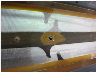
Fig. 3. LQ Inner Layer Protection Heaters show signs of de-lamination
