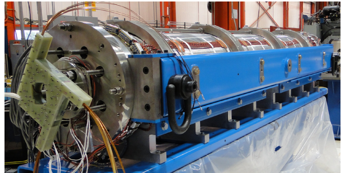
Fig. 1. LQS01 during the preparation of coil interconnections. Bottom raft and side beams are used for handling and are removed before test.
