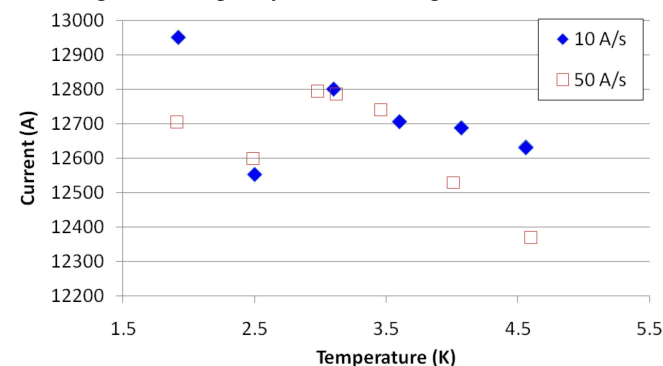
Fig. 6. Highest quench current in LQS01b at different temperatures and ramp rates.
