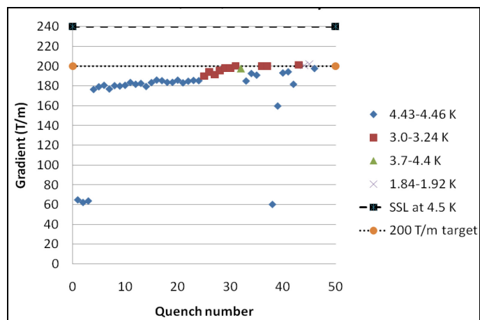
Fig. 2. LQS01a quench history.
