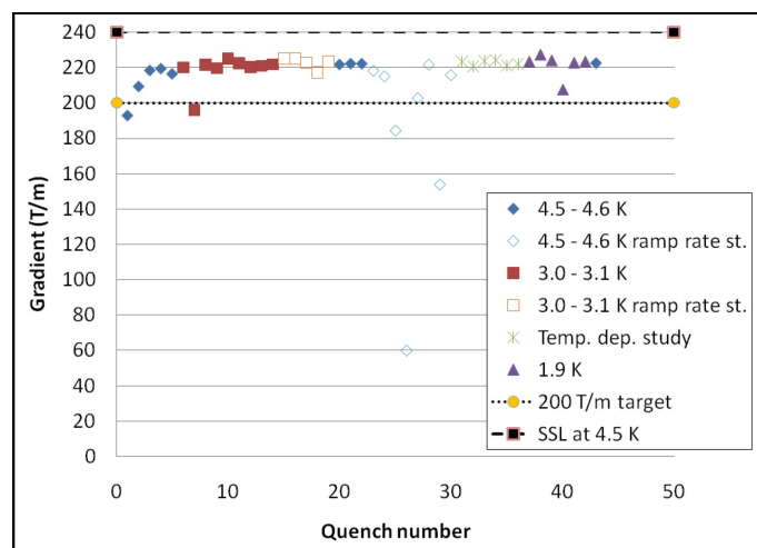
Fig. 4. LQS01b quench history.
