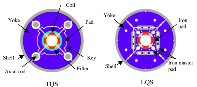
Fig. 1. Schematic view of the TQS and LQS yoked magnets
