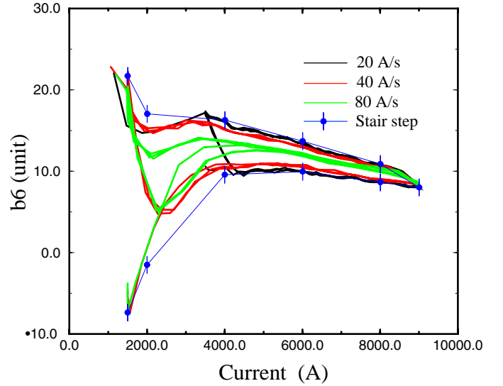
Fig. 4 LQS01 current loops executed at ramp rate of 20, 40 and 80 A/s. The points represents the “stair step” measurement described in the text.
