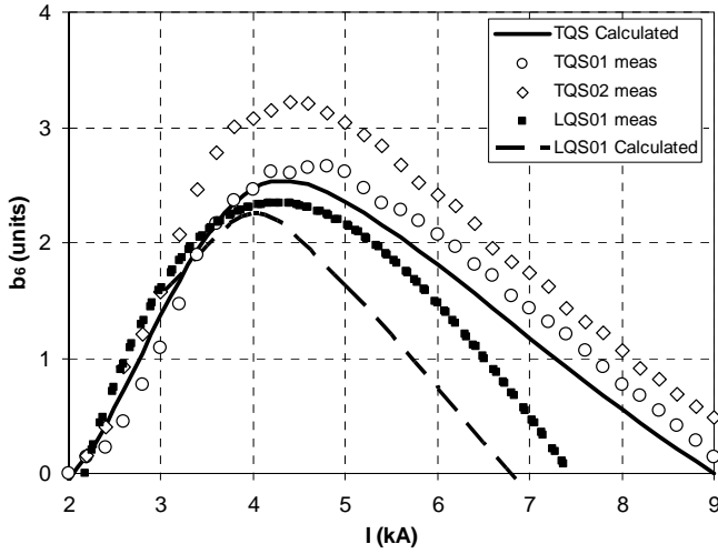
Fig. 3 Iron saturation effect in TQS01-02 and LQS01.
