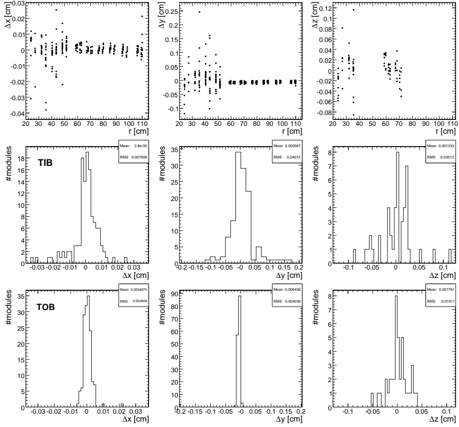
Figure 24. Differences in determined x - (left), y - (centre) and z -positions (right, only double-sided) of active modules comparing the +10 °C and -10 °C configurations. The differences are stated as a function of the module radius r (top row) and for modules in TIB (middle row) and TOB (bottom row) separately.
