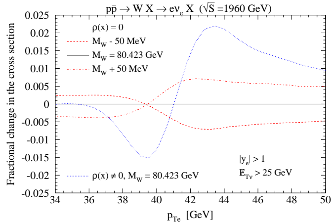
Fig. 4.6.110: The fractional change in the d\sigma/dp_{T_e} distribution in forward W boson production at the Tevatron ( |y_e| > 1 , E_T > 25 GeV) due to the small- x broadening (blue dotted line) [222]. The dashed and dot-dashed lines correspond to \delta M_W = \pm 50 MeV in the case when the broadening is absent.
