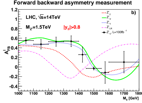
Fig. 4.1.92: The forward-backward asymmetry, A_{FB}(M(l)) , of single Z' production in pp \rightarrow Z' \rightarrow l^+l^- at the LHC for a number of models with heavy, non-standard gauge bosons. Taken from Ref. [188].
