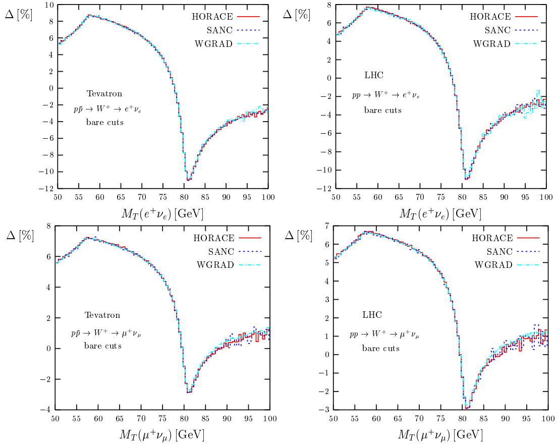
Fig. 4.4.93: The relative correction \Delta due to electroweak \mathcal{O}(\alpha) corrections to the M_T(l\nu) distribution for single W^+ production with bare cuts at the Tevatron and the LHC.
