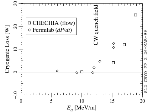
Figure 2. Cryogenic loss measurements with 500 \mu\text{s} fill time and 800 \mu\text{s} flat top at 1 Hz.
