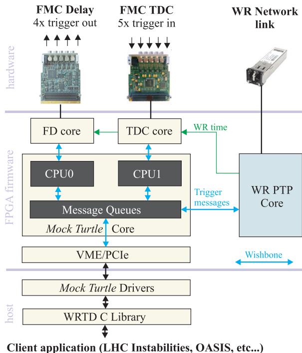
Figure 5: Architecture of the WRD Hardware, FPGA and software.
