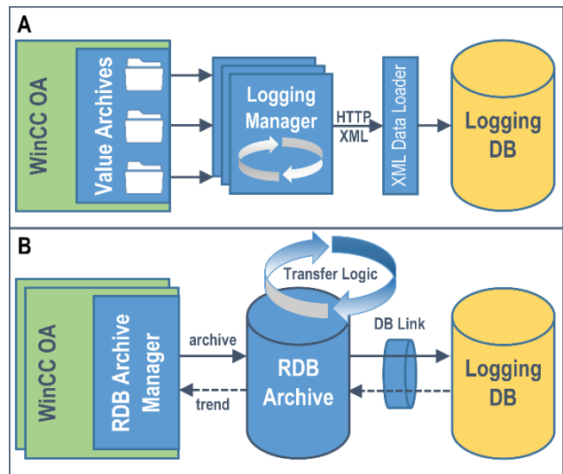
Figure 1: Archiving architecture: (A) with old logging manager; (B) with Oracle archiver and DB-link data transfer.
