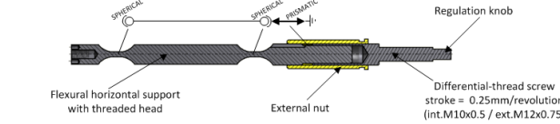
Figure 4: Operating principle of vertical and horizontal supports actuation.
