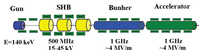
Figure 2: Layout of layout of thermionic gun based injector.
