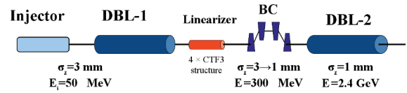
Figure 7: DBL layout with RF gun based injector.
