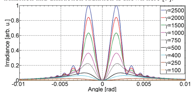
Figure 1: OTR angular distribution calculated by ZEMAX for \lambda=550 nm and for different energies.
