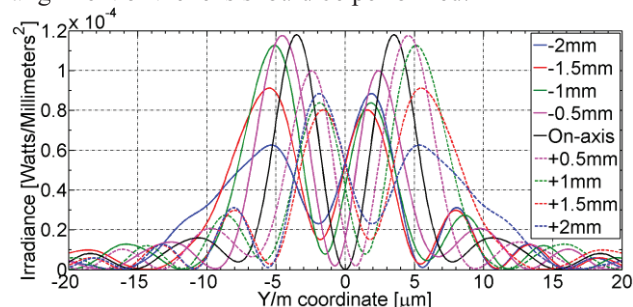
Figure 5: OTR PSF distribution calculated by ZEMAX for different lens offsets ( \lambda=550 nm; \gamma=2,500 ).
