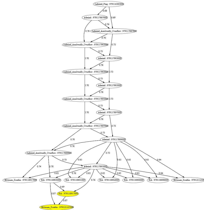
Figure 3: LLDOS1.0 hyper-alerts generated by using updated ACM
