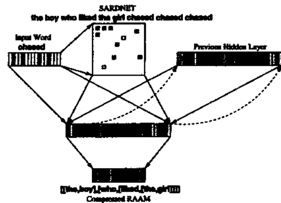
Figure 2: The SARDSRN Network. This snapshot shows the network during step 11 of figure 1. The representation for the current input word, chased, is shown at top left. Each word is input to the SARDNET map, which builds a representation for the sequence word by word. At each step, the previous activation of the hidden layer is copied (as indicated by the dotted line) to the Previous Hidden Layer assembly. This activation, together with the current input word and the current SARDNET pattern, is propagated to the hidden layer of the SRN network. As output, the network generates the compressed RAAM representation of the top element in the shift-reduce stack at this state of the parse (in this case, line 12 in figure 1). SARDSRN is a map of word representations, and is trained through the Self-Organizing Map (SOM) algorithm [Kohonen, 1995; 1990]. All other connections are trained through backpropagation.
