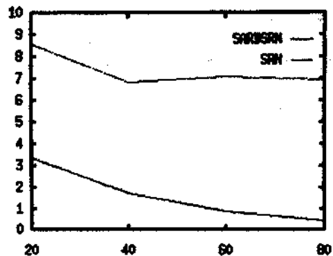
Figure 5: Results. Averages over four simulation runs using the stricter average mismatches per sentence measure on the test data. The SRN's performance in all 16 runs bottomed out at a much higher error than SARDSRN, while still unable to parse all of the training sentences. SARDSRN, on the other hand, did learn to parse the training sentences, and showed very good generalization to the test sentences. These differences are statistically significant with p < 0.0005 .
