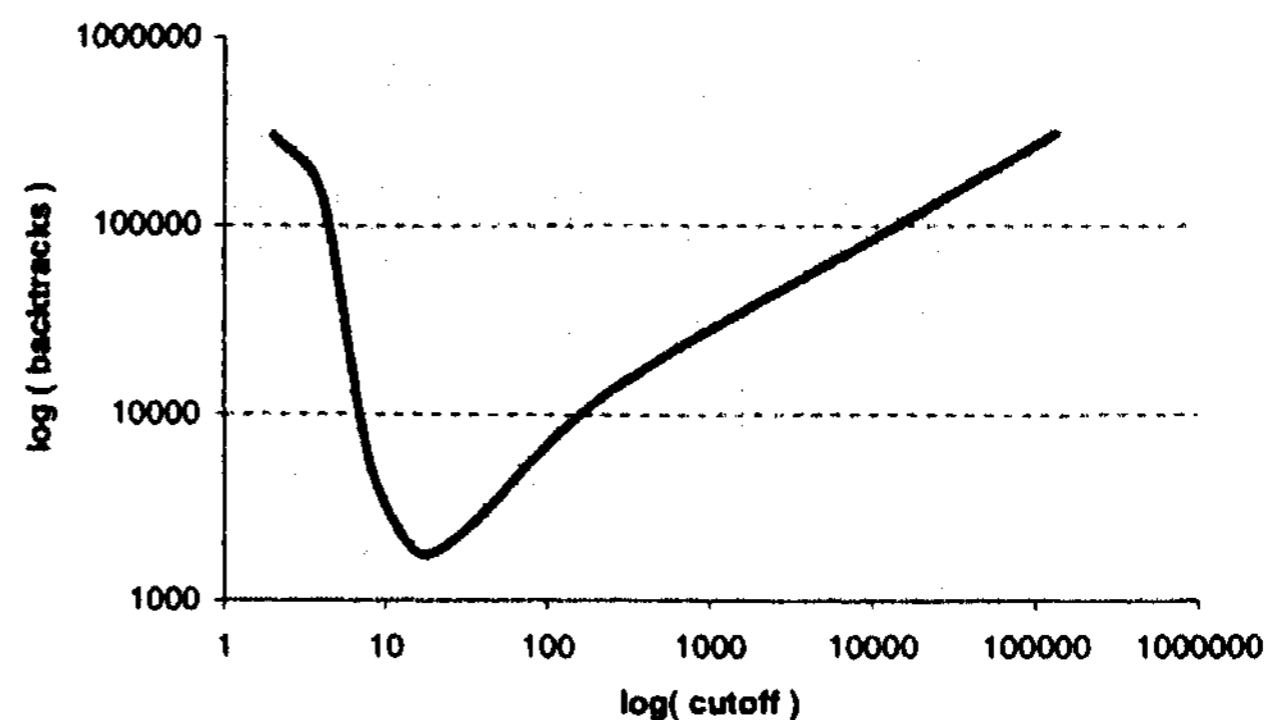
Figure 1: Relationship of the cutoff value (measured in backtracks until a restart is performed) on expected solution time. Data is for a randomized backtracking algorithm (satz-rand) for the SATPLAN encoding of a logistics planning problem (log.d). The Y-axis specifies the expected number of backtracks performed until a solution is found, counting the previous failed restarts.
